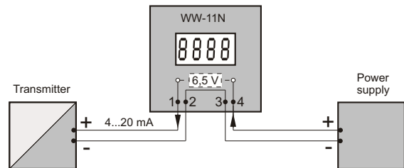
Electrical diagram
