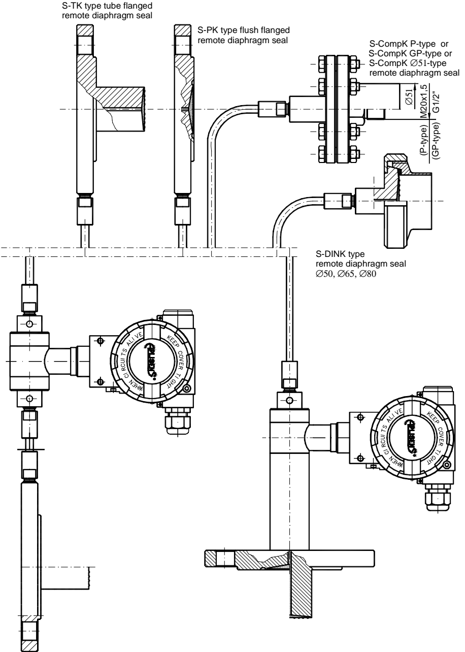
Fig. 14. APR-2200ALW differential pressure transmitter with two remote diaphragm seals (examples)
