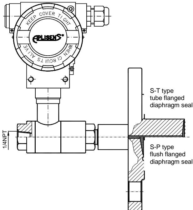
Fig. 10. APR-2000ALW differential pressure transmitter with a single direct diaphragm seal (example).
