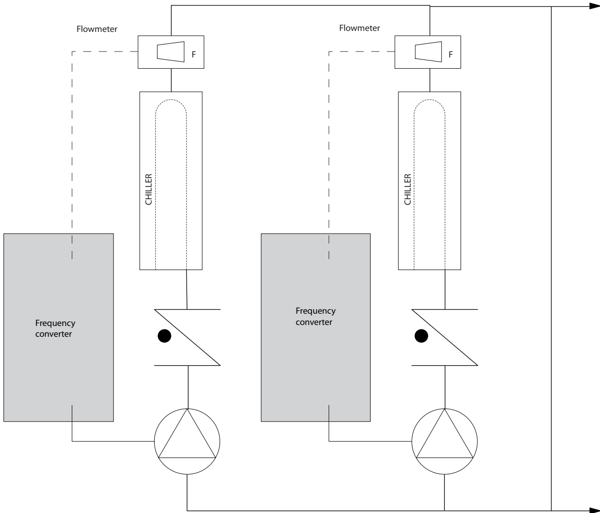
Illustration 5.20 Drives Used with Primary Pumps in a Primary/Secondary Pump System
