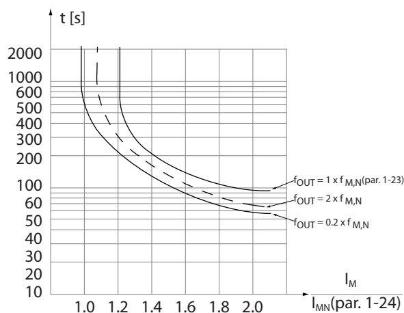
Illustration 5.1 ETR Characteristics
