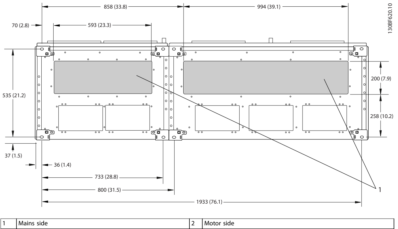
Illustration 8.81 Gland Plate Dimensions for F12
