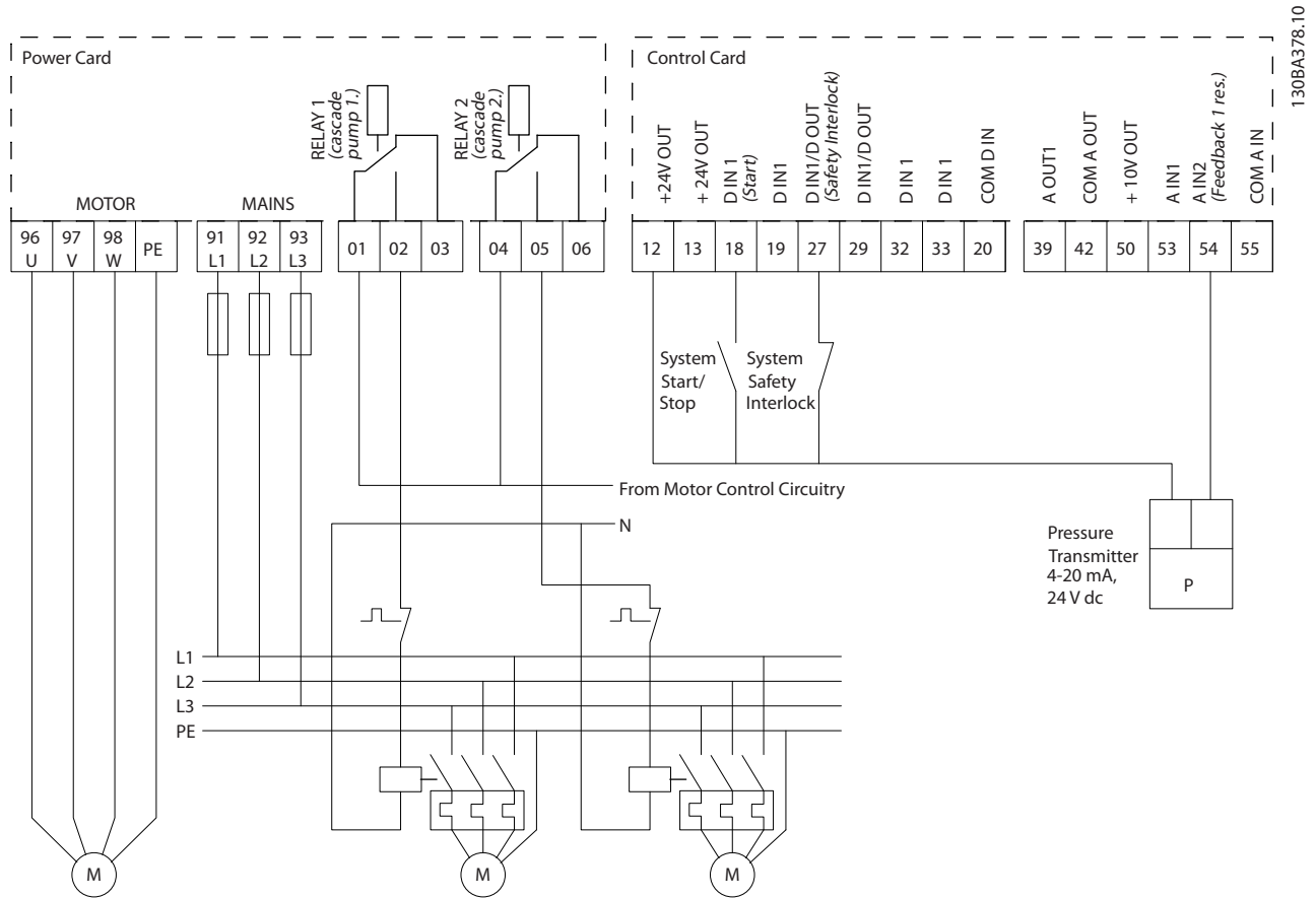
Illustration 12.4 Cascade Controller Wiring Diagram
