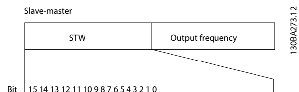
Illustration 14.17 STW Slave-to-Master
