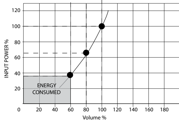
Illustration 5.7 Energy Saved with Reduced Fan Capacity
