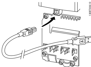
Illustration 10.6 USB Connection
