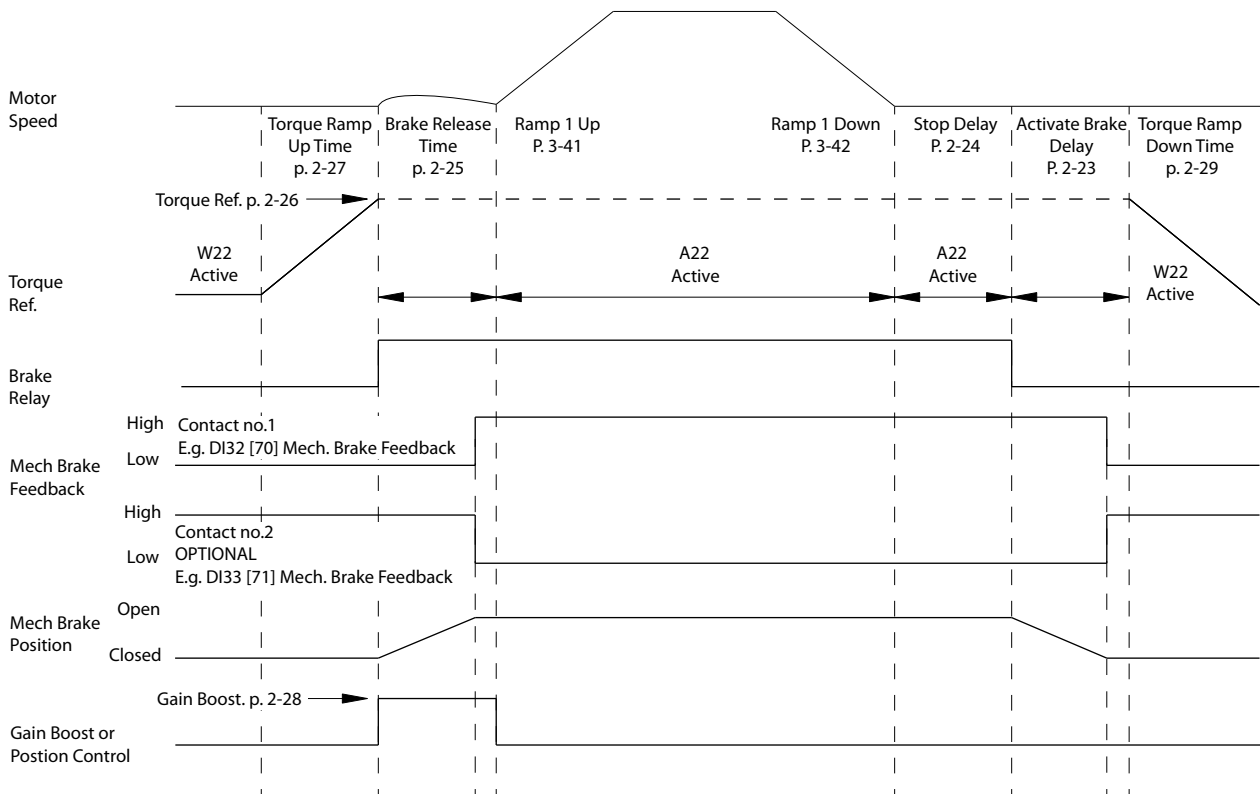
Illustration 5.8 Brake Release Sequence for Hoist Mechanical Brake Control
