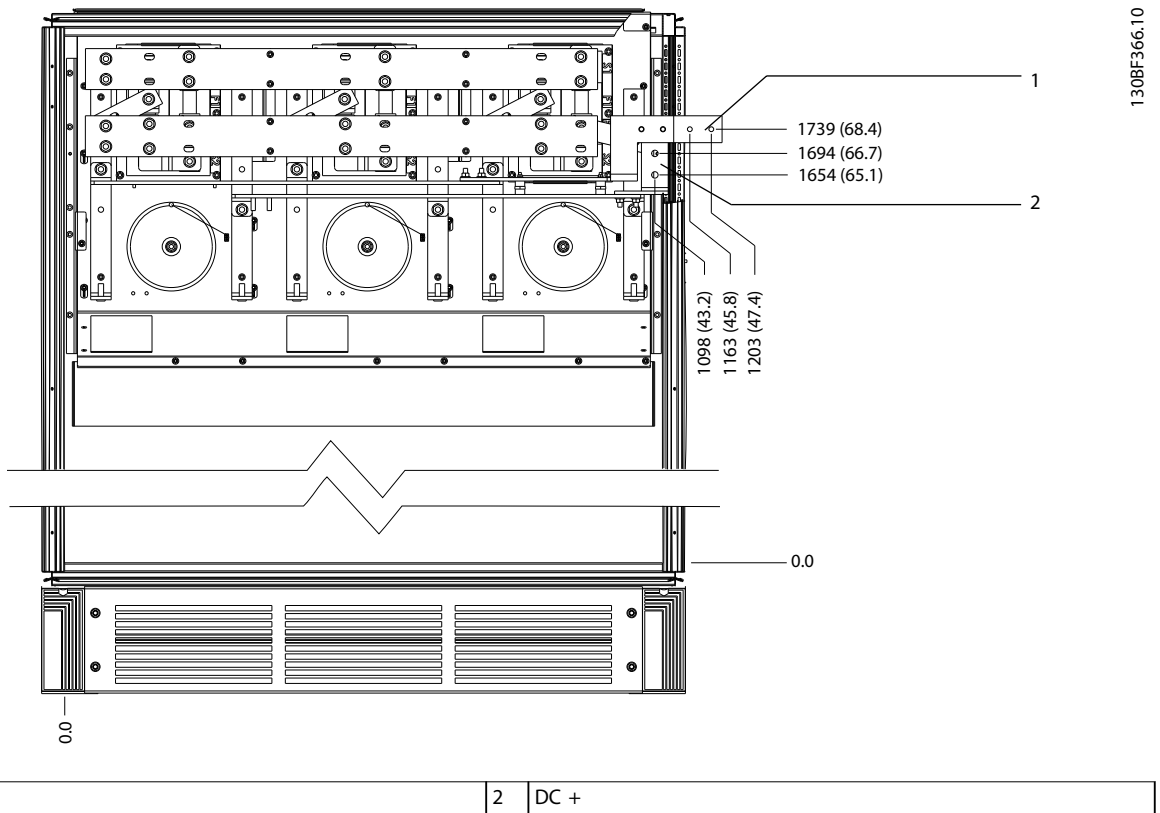
Illustration 8.55 Terminal Dimensions for F2/F4 Regeneration Terminals, Front View
