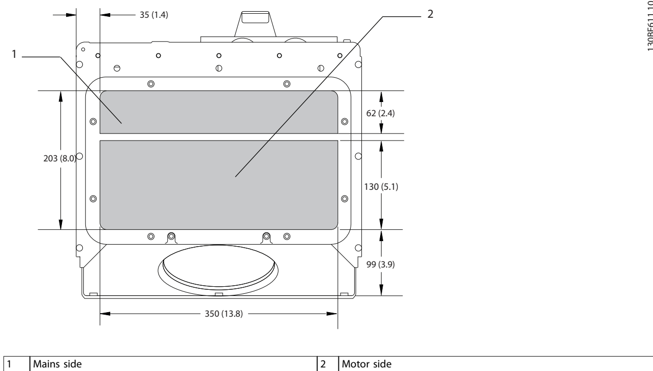
Illustration 8.2 Gland Plate Dimensions for E1/E2
