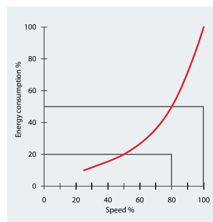
On fan and pumps up to 50% energy can be saved by reducing the speed from 100% to 80%.
