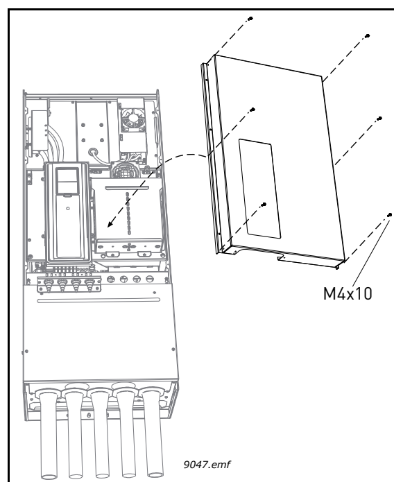
Figura 46. Reinstalar a tampa principal (MR9)
