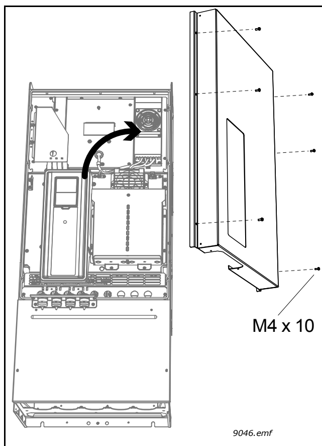
Figura 33. Retirar a tampa principal (MR9)
